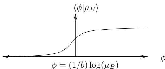
Figure 1: Illustration of profile \langle \phi | \mu_B \rangle \sim e^{-\mu_B e^{-b\phi}} of the boundary state |\mu_B\rangle
